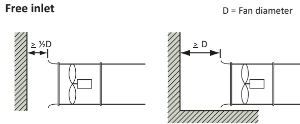
Optimum installation
