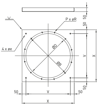
Vertical mounting plate for AZN-AZW with Ø350 and Ø560 hubs
