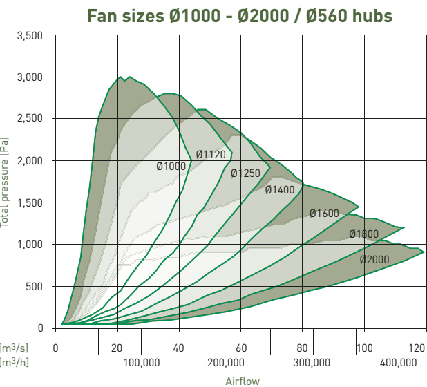
Specific performance curves for fans with frequency drives
