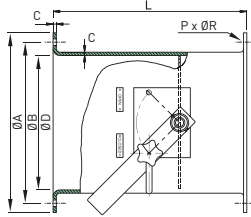
Damper type SBC
